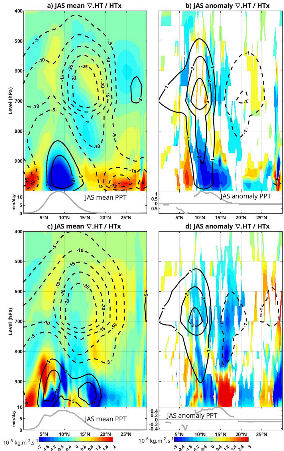
Figure 8. July, August, and September 1978–2018 ERA5 reanalyzes, average (left) and linear regressions on the PCICRU index (right) in vertical meridional sections over the ocean (22°W–17°W, (a, b)) and over the continent (10°–5°W, (c, d)): Divergence of moisture transport (colors) and zonal moisture transport (black contours, solid for positive, dashed for negative), superimposed on precipitation (gray line in panels at the bottom). Only values significant at the 95% confidence level are plotted.
